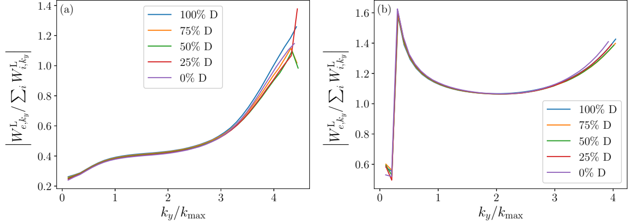
Figure 15: Linear energy weight magnitude ratios |W_{e,k_y}^L/\sum_i W_{i,k_y}^L| for different relative concentrations of D and T against k_y/k_{\max} for the GA-std case (a) and the a/L_n = 3.0 case (b). Note the essential invariance across the spectrum for the different concentrations.
