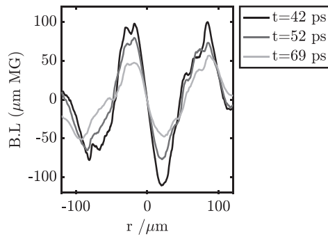
FIG. 5. B_x L along the axis of symmetry of the magnetic fields for shot B shown in Fig. 4.
