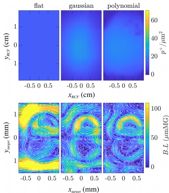
FIG. 8. Field retrievals (bottom row) at the interaction plane of t = 33 ps film in Fig. 4 using different assumed “undisturbed” proton flux distributions shown at the detector plane (top row) including, from left to right, a flat mean-field, a \sigma = 150 -pixel Gaussian filter with 200-pixel kernel size, and a custom 2D 3rd-order polynomial, masked with the beam edge, in which the low flux regions are replaced with the original image.
