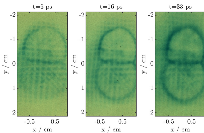
FIG. 3. RCF of the early time evolution of the proton deflectometry. The laser focal spot separation was 820\text{ }\mu\text{m} . The RCF layers, from left to right, correspond to proton energies of 5.6\text{ MeV} , 4.6\text{ MeV} , and 3.3\text{ MeV} . The image contrast has been adjusted to enhance the proton beam structure.
