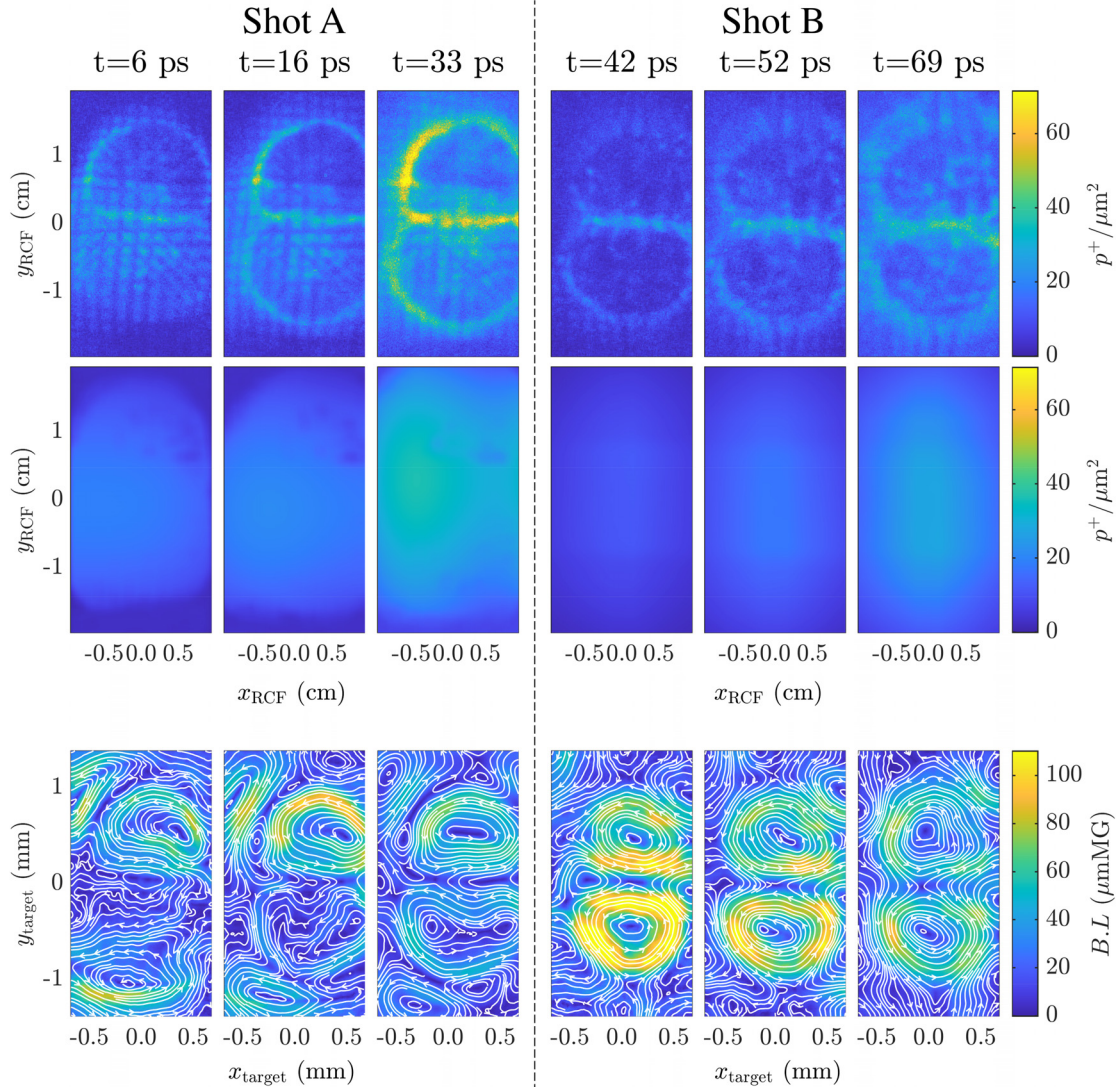
FIG. 4. Time series of magnetic field retrieval, showing the measured protons/ \mu\text{m}^2 at the detector plane (top row), the calculated undisturbed beam flux at the detector plane (middle row), and retrieved path-integrated magnetic fields at the interaction plane (bottom row) for the increasing time after arrival of the laser (left to right). The white contours with arrows show the topology of the calculated magnetic fields. The time series is composed of films from two separate shots, three early times from shot A (left), and three later times from shot B (right).
