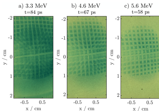
FIG. 7. Measure proton distributions for (a) 3.3 MeV, (b) 4.6 MeV, and (c), 5.6 MeV protons (the same energies as the films in Fig. 4) that have not interacted with the reconnection target. This illustrates the “innate” distortion of the mesh.
