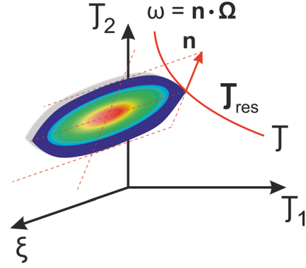
Figure 1. A phase space island near the resonant surface, \mathbf{n} \cdot \Omega(\mathbf{J}) = 0 .
