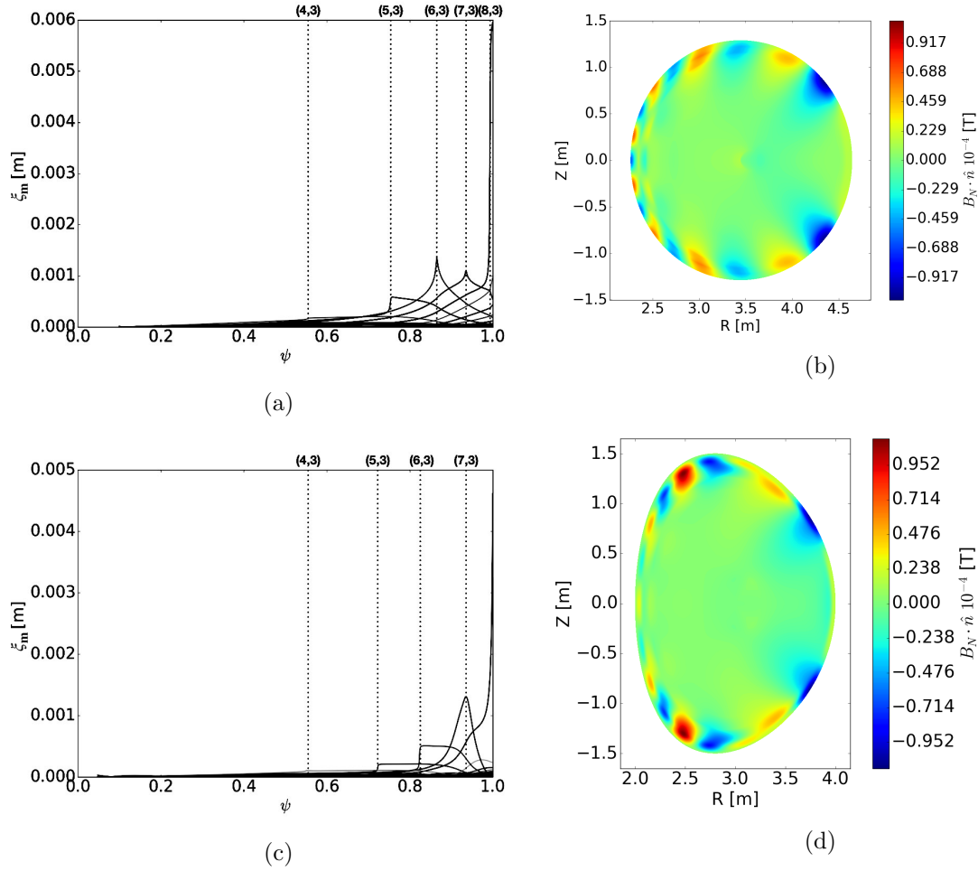
Figure 2: Linear, ideal MHD plasma response to an applied N = 3 even MP. The radial dependence of the straight field line poloidal harmonics of the normal displacement functional \xi_N \cdot \nabla\psi [m] for the (a) circular ( cbm18_dens6 ) and (c) D-shaped ( dbm9 ) equilibrium. The reconstruction in the poloidal cross-section of the normal magnetic field B_N \cdot \hat{n} [T] for the (b) circular ( cbm18_dens6 ) and (d) D-shaped ( dbm9 ) equilibrium.
